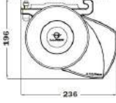
Top-fix
