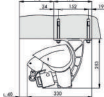
Top-fix
